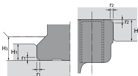
Shoulder for the LM Rail
